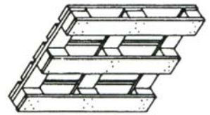
Block, Double Face, Flush 4-Way Entry, Europallet _____
